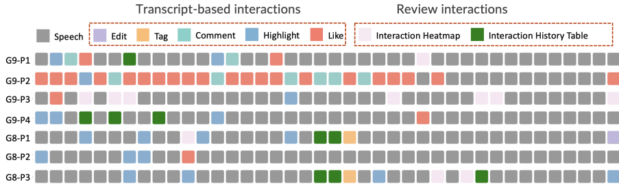
Fig. 8. The most frequently used interactions changed over time in two example sessions. Participants used transcript-based interactions more often in the first three-quarters of the discussion when there were emerging new ideas.
