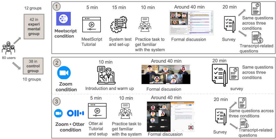
Fig. 6. The participants were randomly assigned to the three conditions, MeetScript, Zoom, and Zoom+Otter.ai. All users across the three conditions had the same discussion task. Teams in MeetScript and Zoom+Otter.ai received a tutorial on how to use the system at the beginning. Then all teams had their discussion task. Post the discussion, and all teams answered a survey. The survey for MeetScript and Otter.ai conditions contained extra questions about the transcript.
