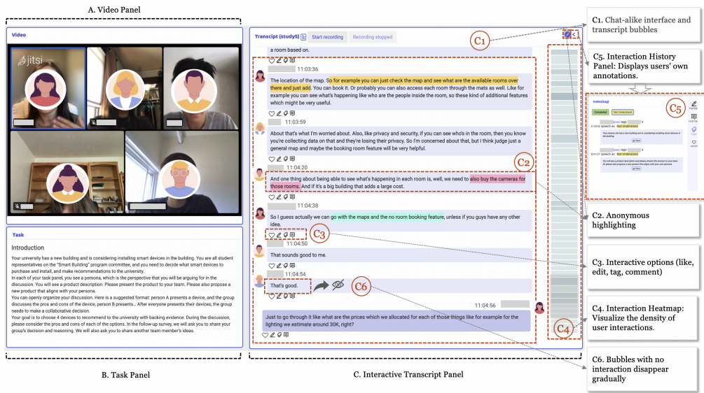
Fig. 1. MeetScript User Interface. MeetScript supports group video meetings through (A) a Video Panel and (C) an Interactive Transcript Panel. Users' conversations are transcribed in real-time and displayed in a chat-alike interface through transcript bubbles (C1). Users have a suite of options to interact and contribute to the conversation unobtrusively through the transcript. Users can highlight (C2), like, edit, tag, and comment on each transcript bubble (C3). To help users process the most essential information, transcript bubbles without user interaction gradually disappear over time (C6). Users can navigate the transcript using the Interaction Heatmap (C4) and Interaction History Panel (C5).
